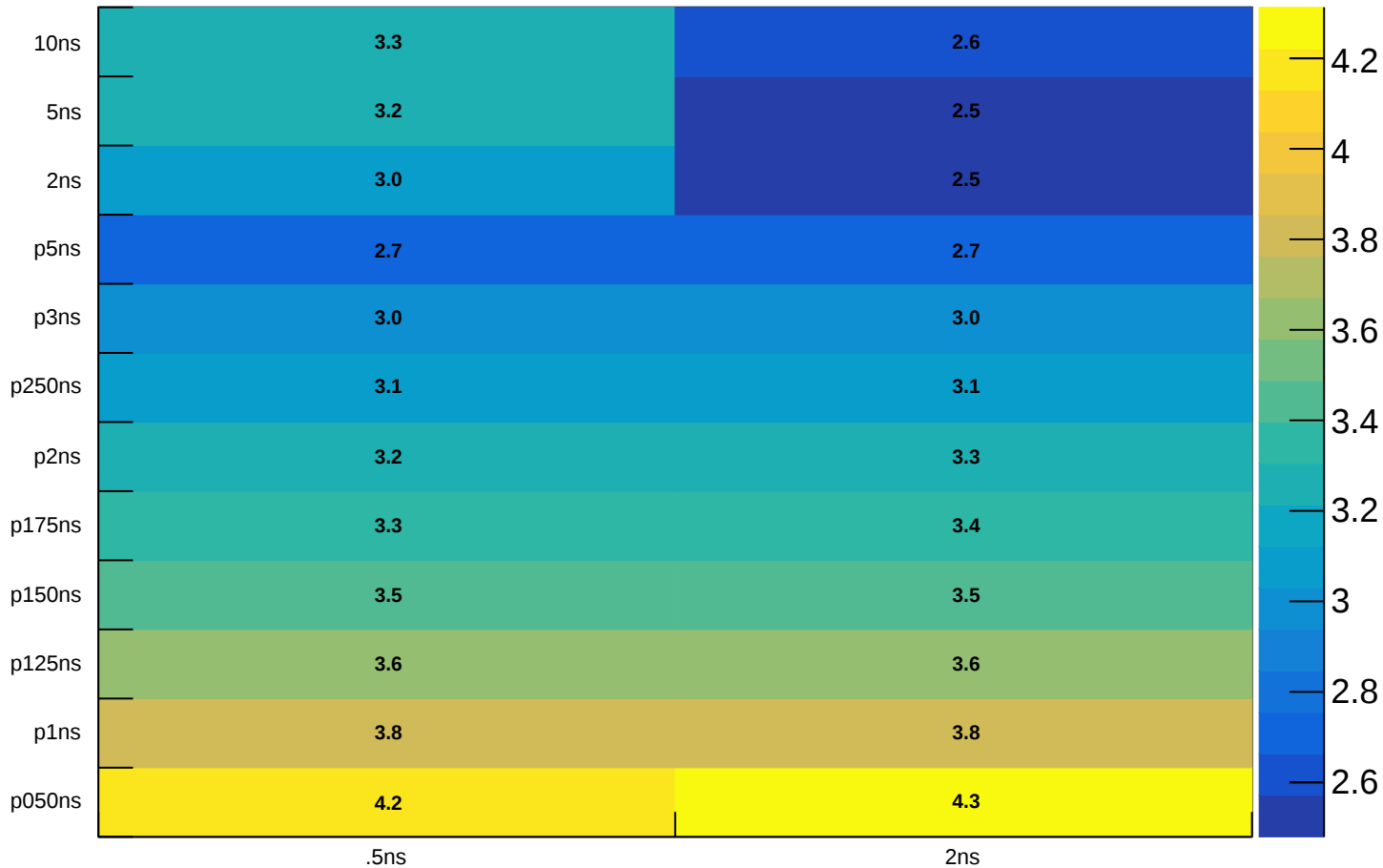
Statistical Significance, highest timing bins [60GeV +.5GeV]
