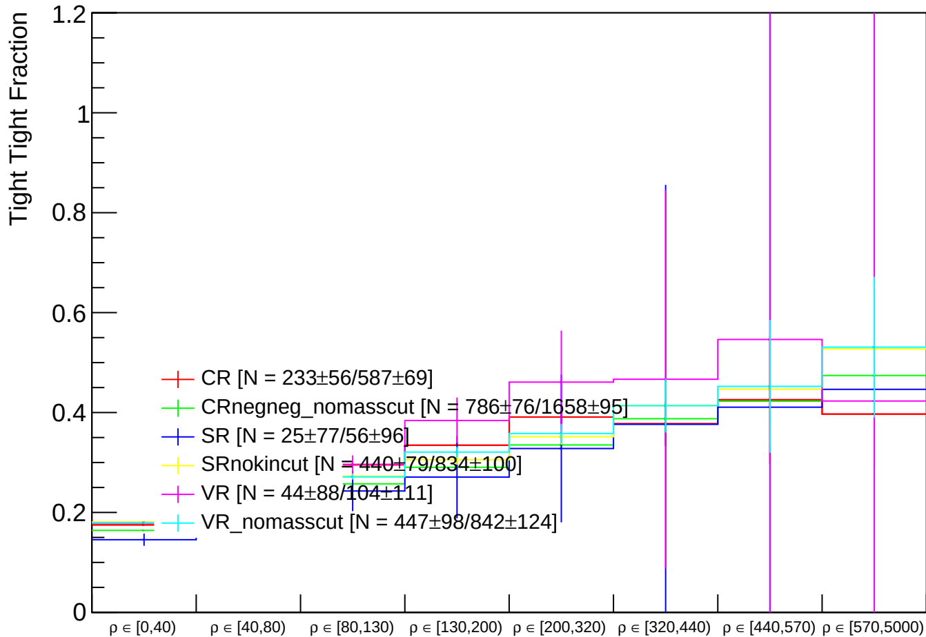
Photon Purity vs \rho
