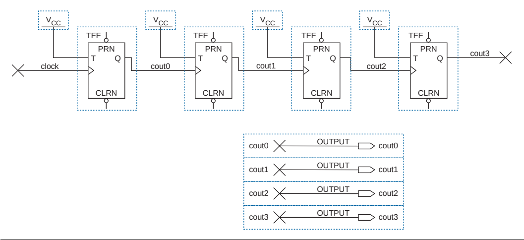
Figure 3–3. 4-Bit Counter Example
