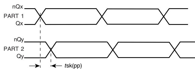
PART-TO-PART SKEW
