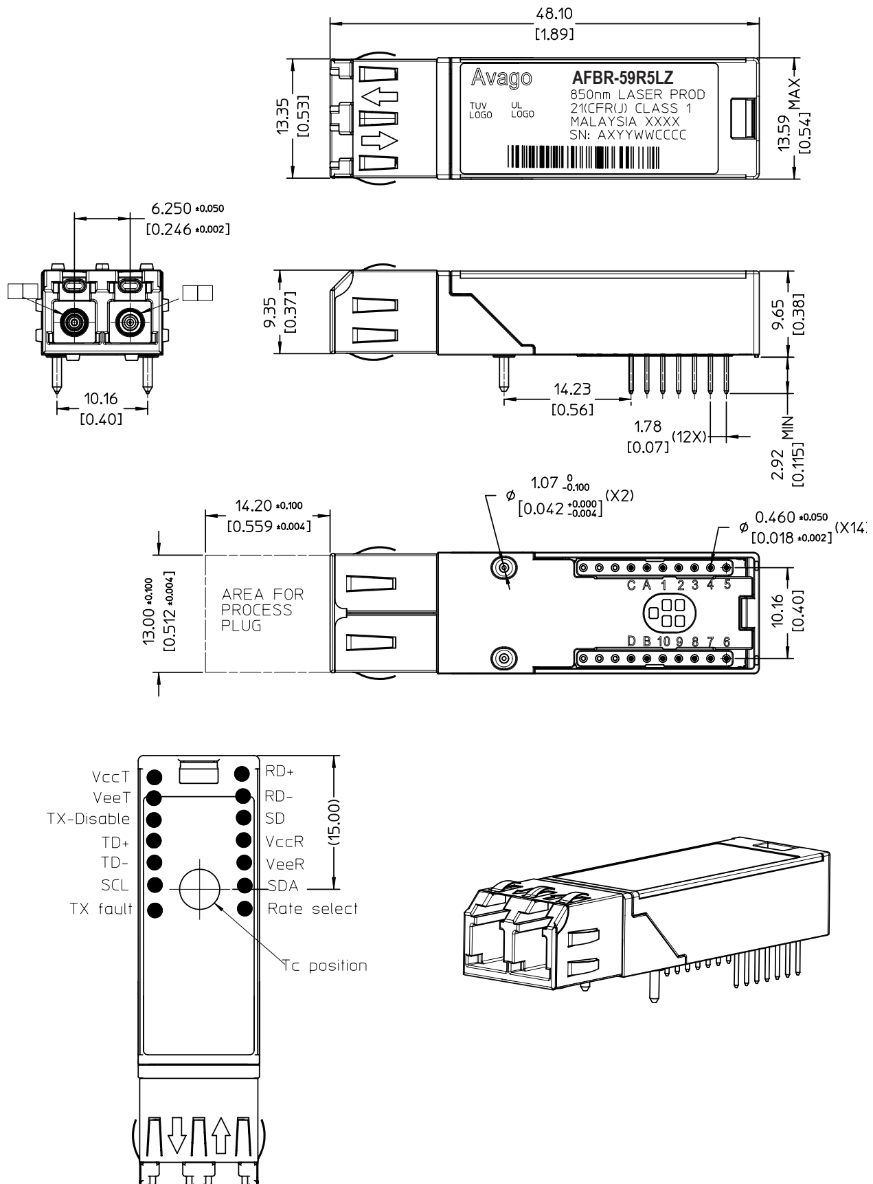
Figure 6. Mechanical Drawing - AFBR-59R5LZ
