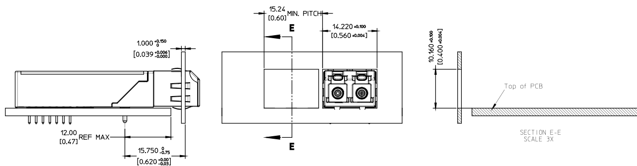
Figure 8. Assembly Drawing
