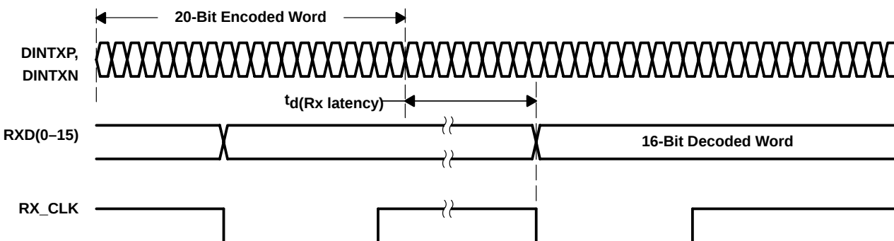
Figure 5. Receiver Latency
