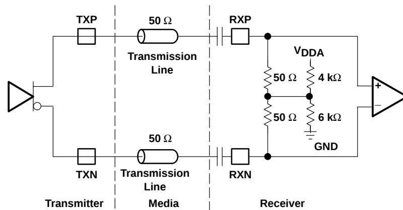
Figure 15. High-Speed I/O AC-Coupled Mode
