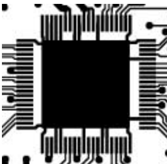
Figure 16. Example of a Thermal Land
