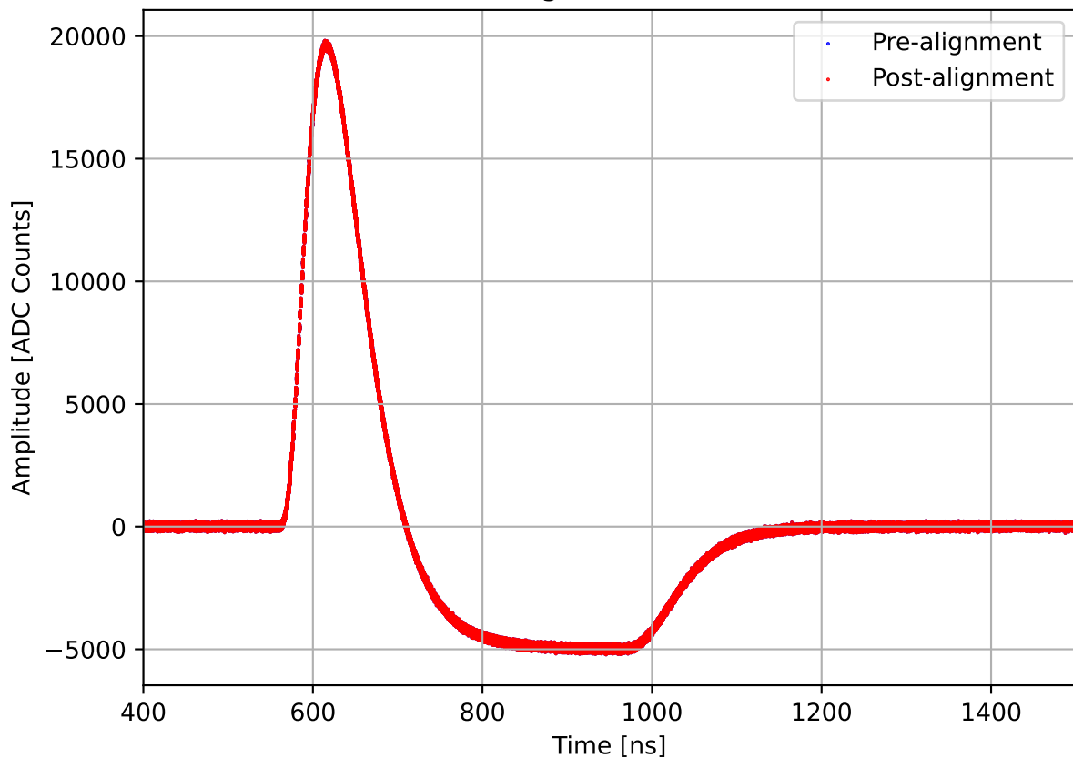
Run 1978, channel7, hi gain, Pulse w/ 0.0 dB Attenuation
