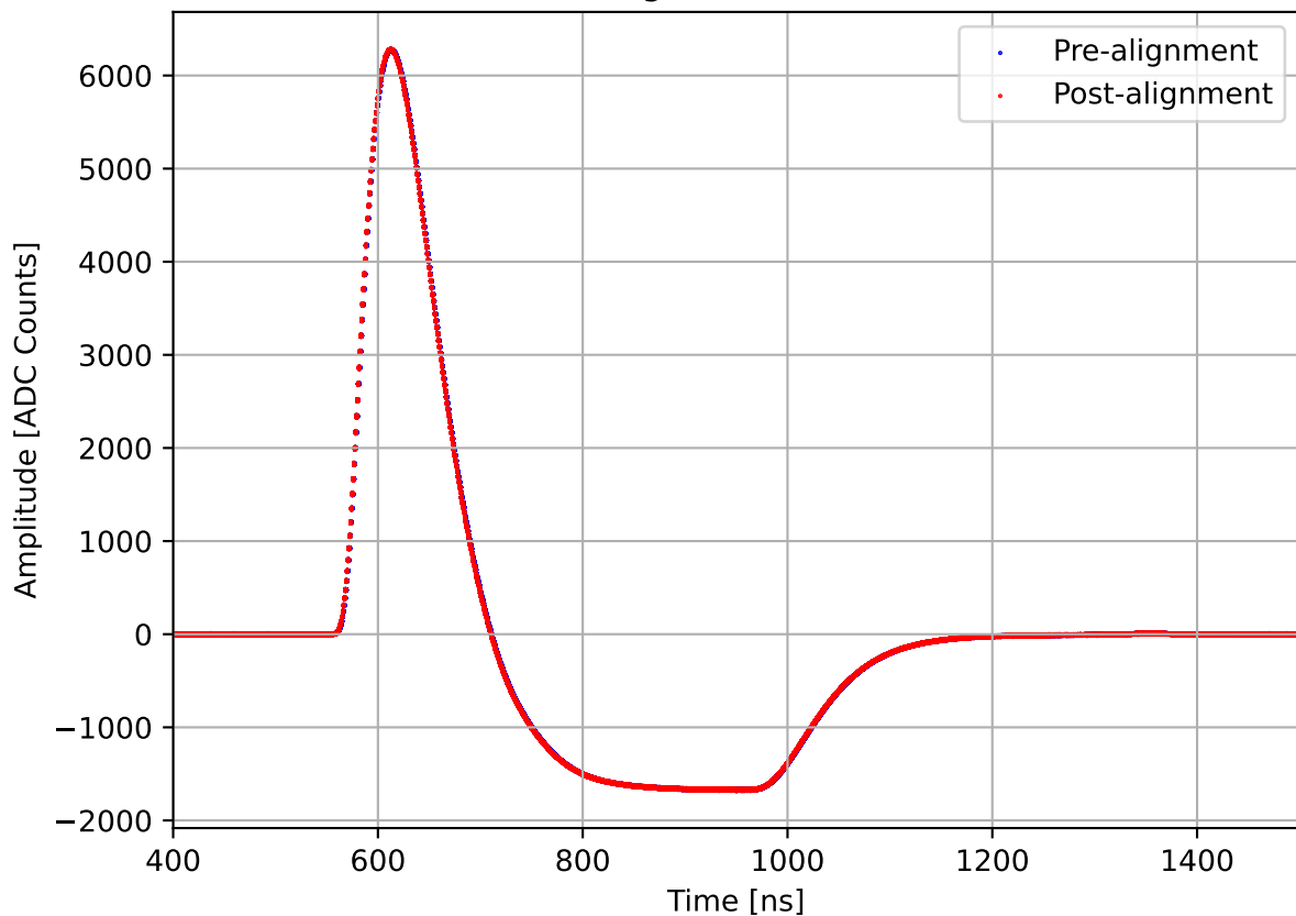
Run 1979, channel8, lo gain, Pulse w/ 10.0 dB Attenuation
