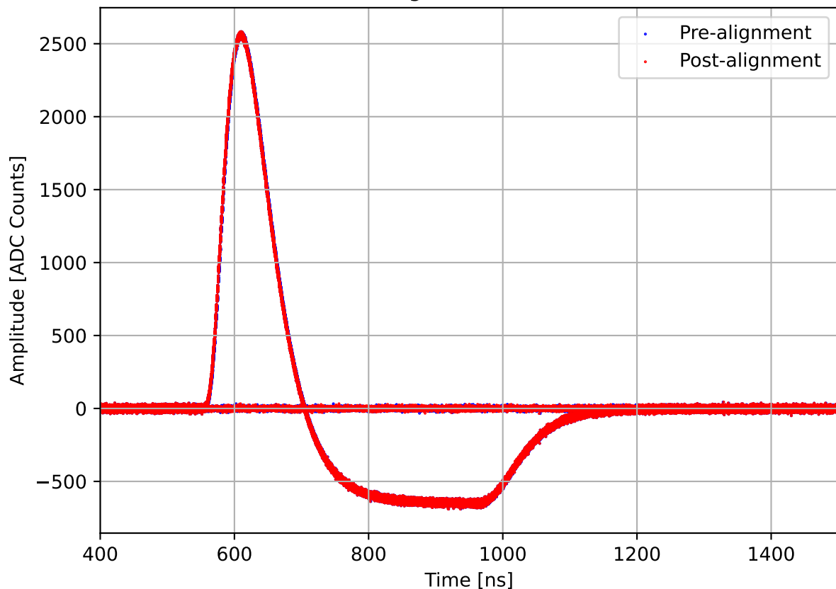
Run 1986, channel7, hi gain, Pulse w/ 40.0 dB Attenuation
