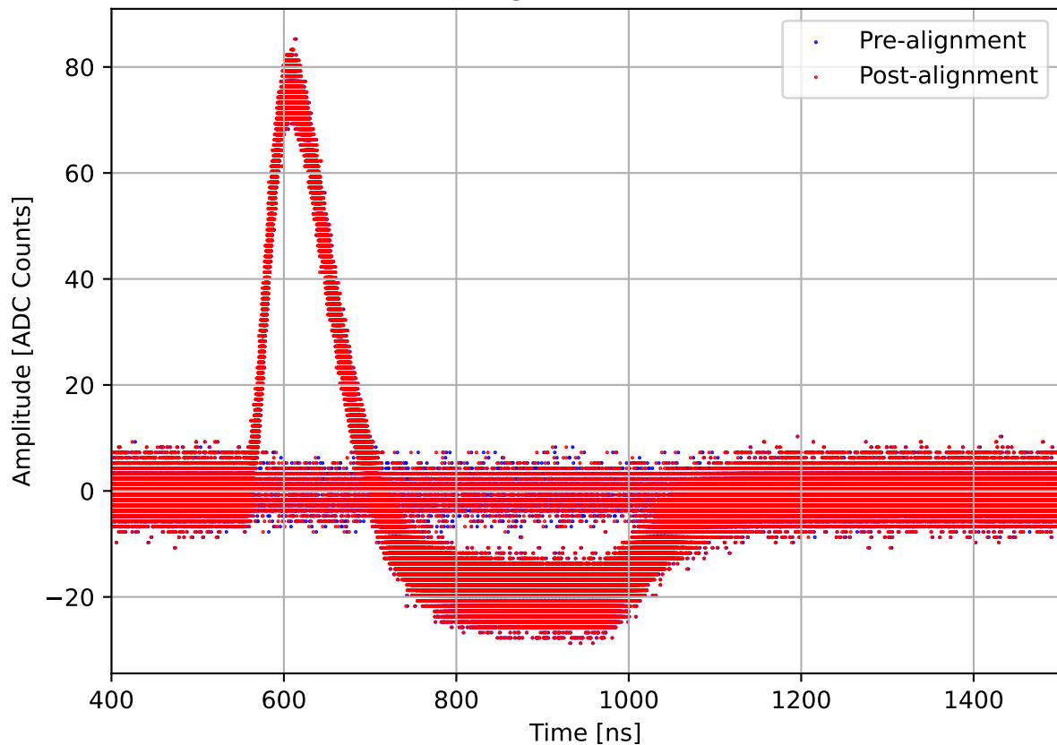
Run 1986, channel8, lo gain, Pulse w/ 40.0 dB Attenuation
