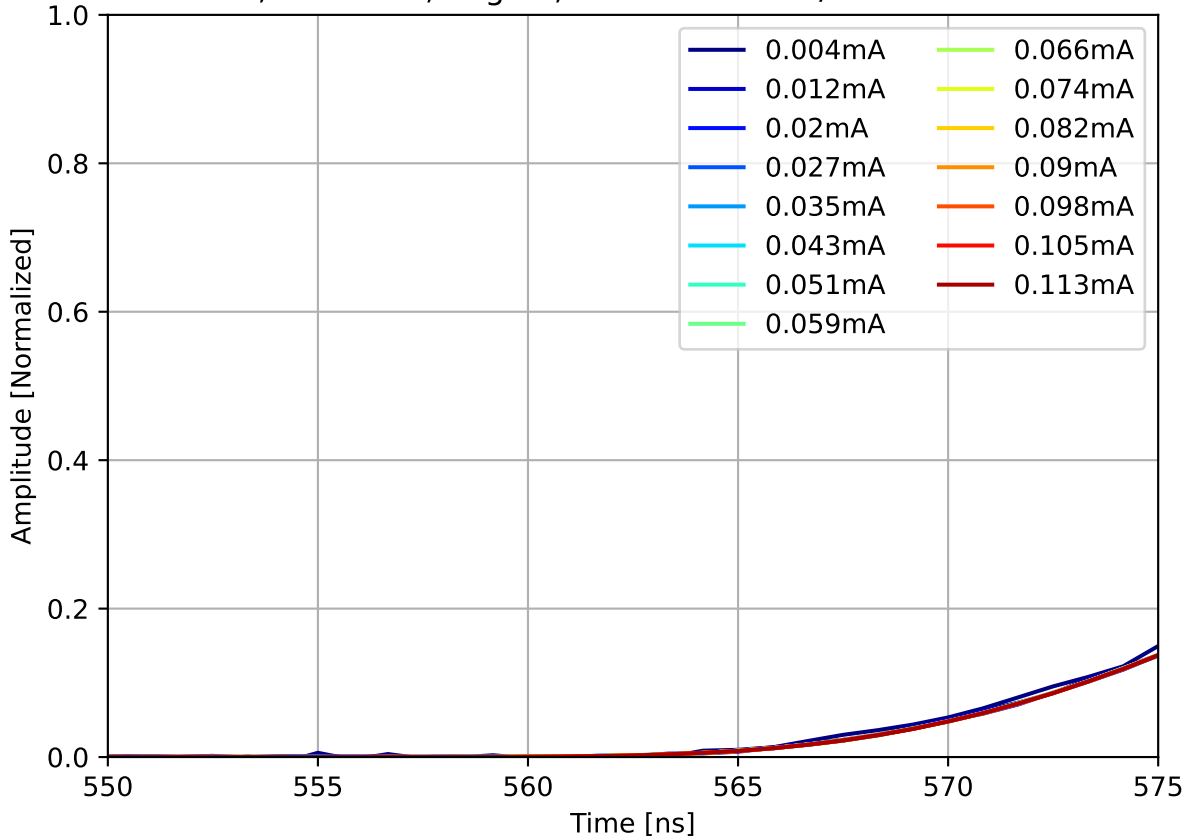
Run 1986, channel7, hi gain, Norm. Pulses w/ 40.0 dB Attenuation
