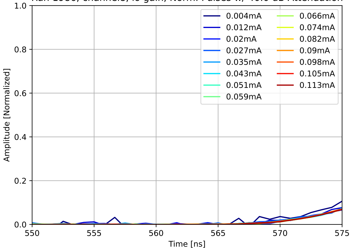
Run 1986, channel8, lo gain, Norm. Pulses w/ 40.0 dB Attenuation
