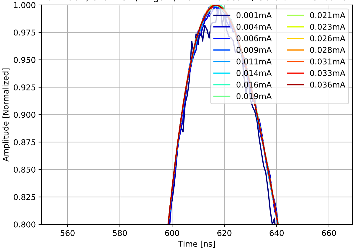
Run 1987, channel7, hi gain, Norm. Pulses w/ 50.0 dB Attenuation
