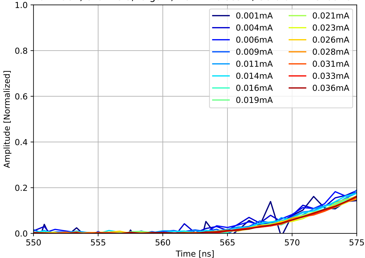
Run 1987, channel8, lo gain, Norm. Pulses w/ 50.0 dB Attenuation
