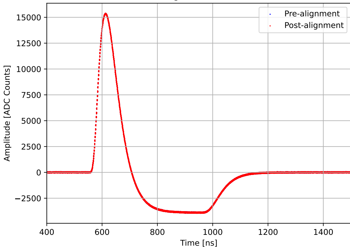
Run 1992, channel7, hi gain, Pulse w/ 12.0 dB Attenuation
