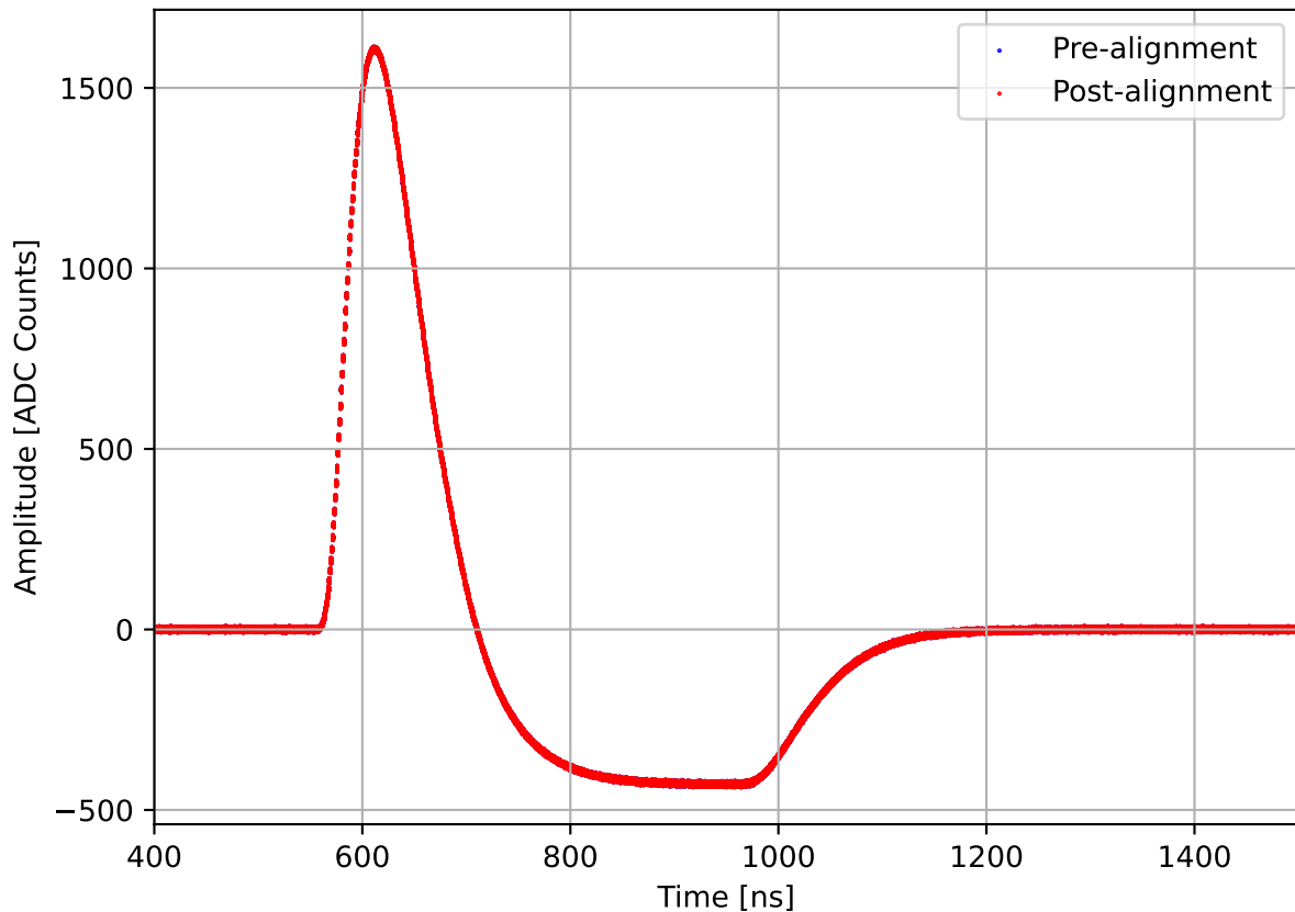
Run 1998, channel8, lo gain, Pulse w/ 17.0 dB Attenuation
