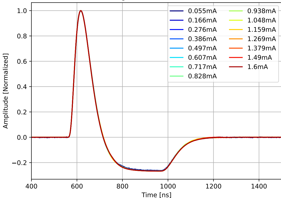
Run 1998, channel8, lo gain, Norm. Pulses w/ 17.0 dB Attenuation
