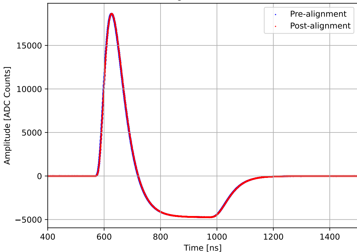
Run 1999, channel7, hi gain, Pulse w/ 27.0 dB Attenuation
