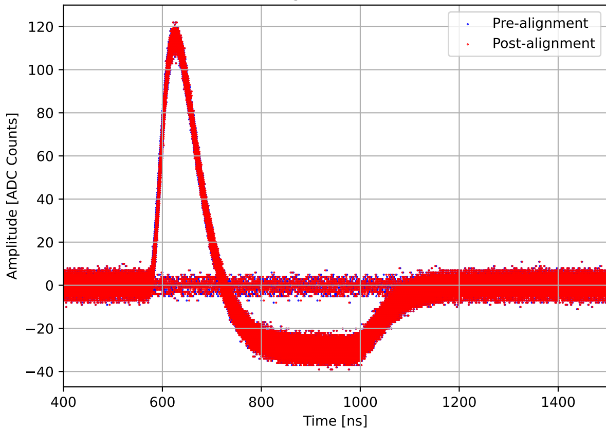
Run 1999, channel8, lo gain, Pulse w/ 27.0 dB Attenuation
