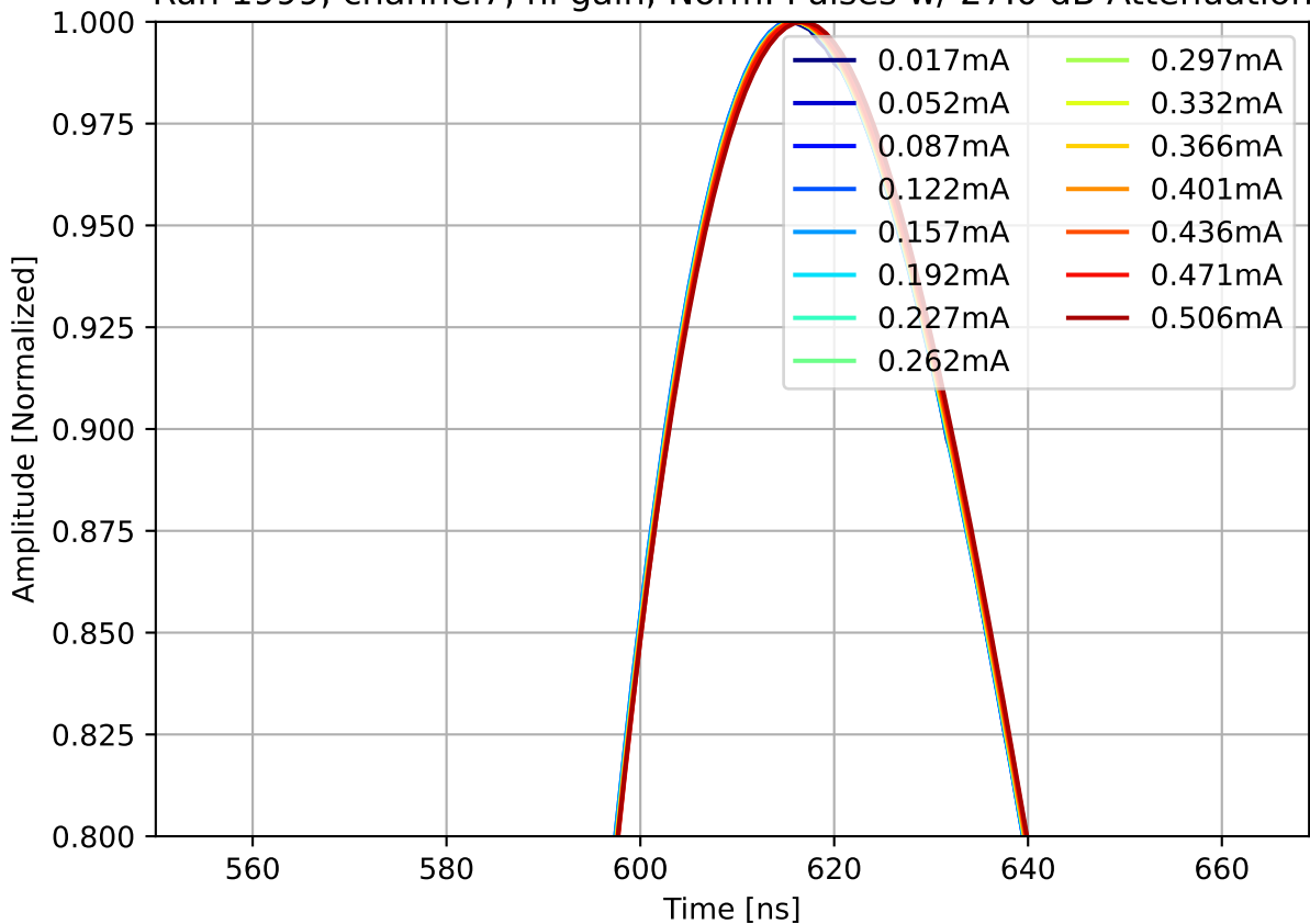
Run 1999, channel7, hi gain, Norm. Pulses w/ 27.0 dB Attenuation
