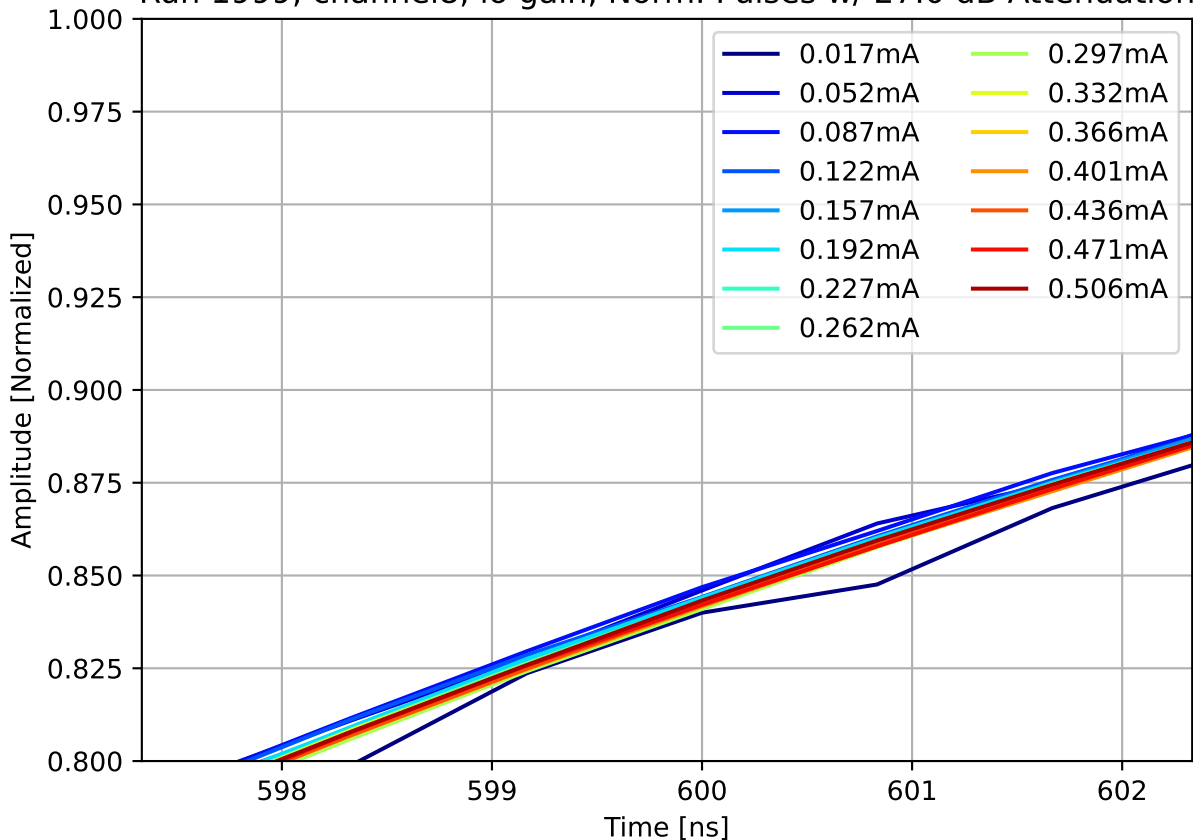
Run 1999, channel8, lo gain, Norm. Pulses w/ 27.0 dB Attenuation
