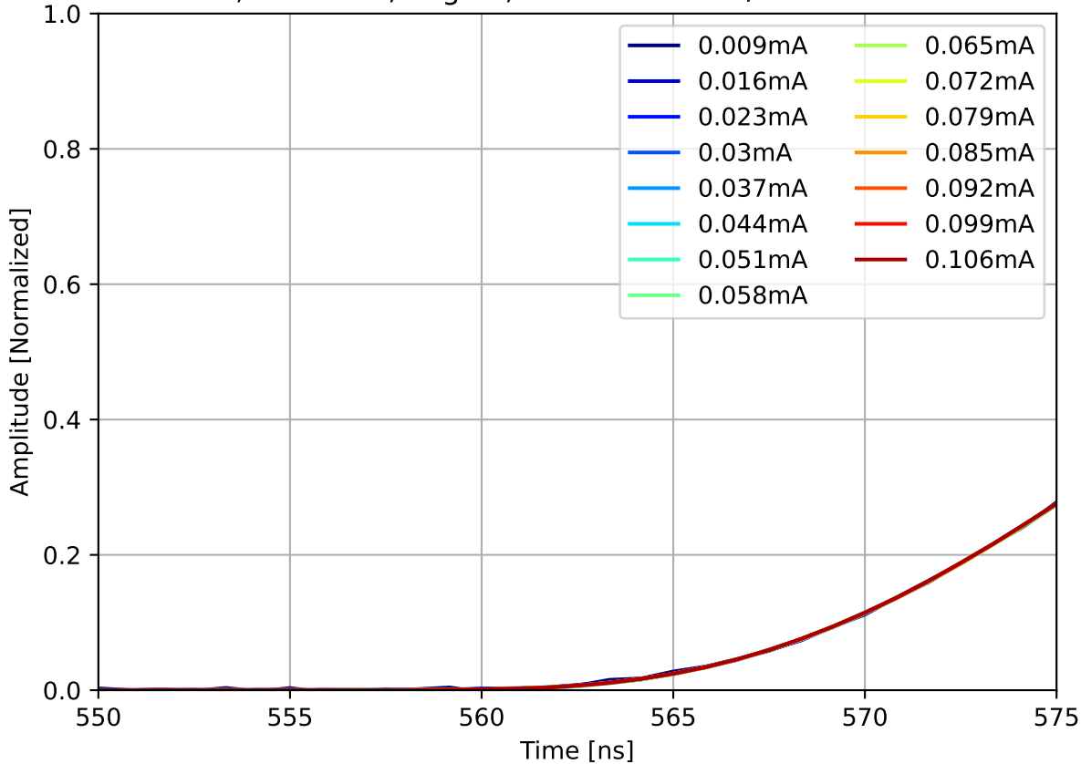
Run 2043, channel5, lo gain, Norm. Pulses w/ 27.0 dB Attenuation
