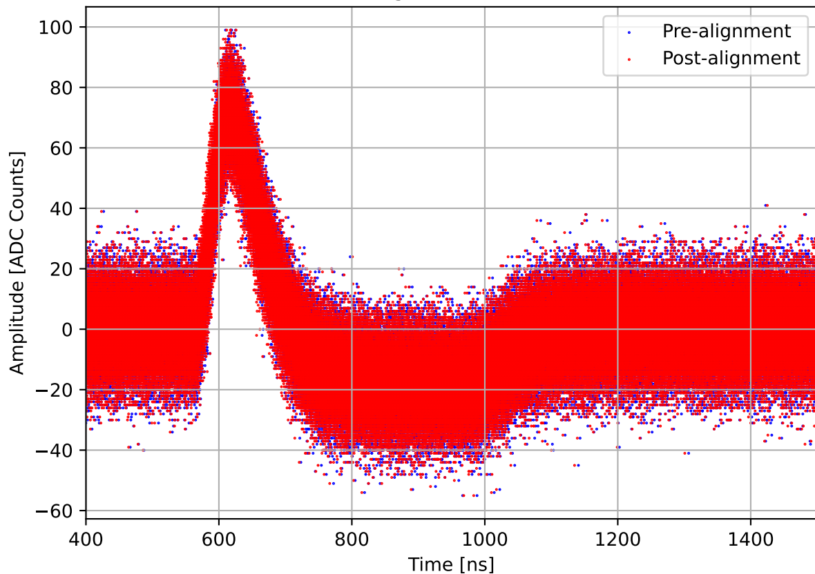
Run 2049, channel7, hi gain, Pulse w/ 70.0 dB Attenuation
