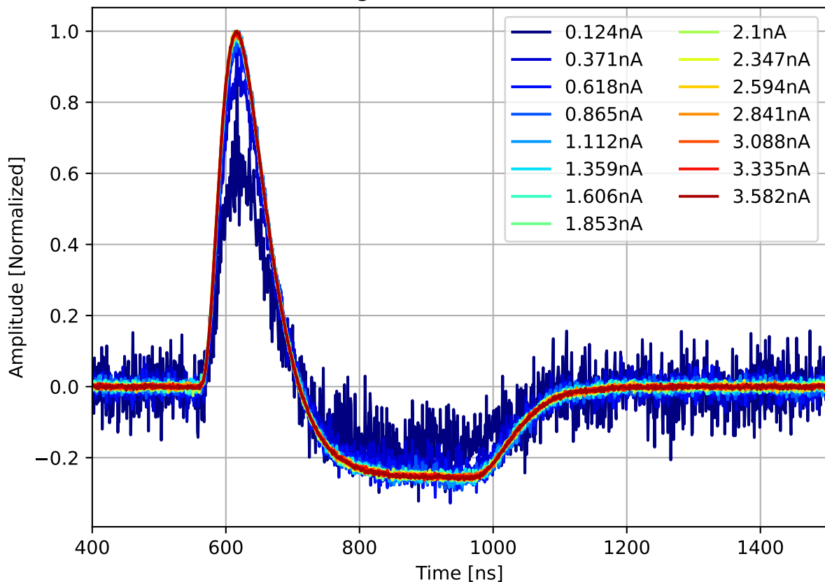
Run 2049, channel7, hi gain, Norm. Pulses w/ 70.0 dB Attenuation
