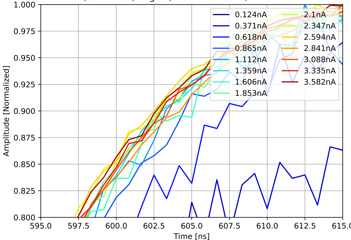
Run 2049, channel7, hi gain, Norm. Pulses w/ 70.0 dB Attenuation
