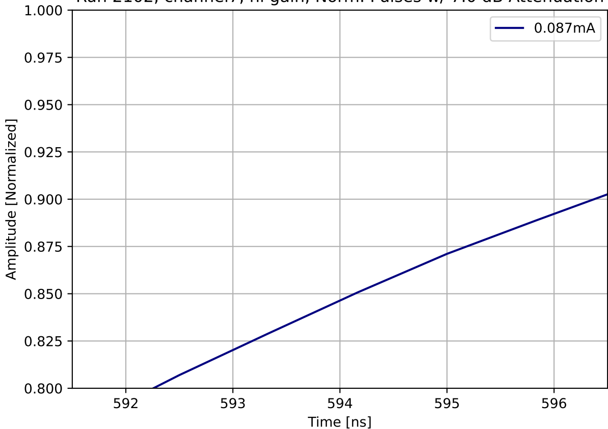
Run 2102, channel7, hi gain, Norm. Pulses w/ 7.0 dB Attenuation
