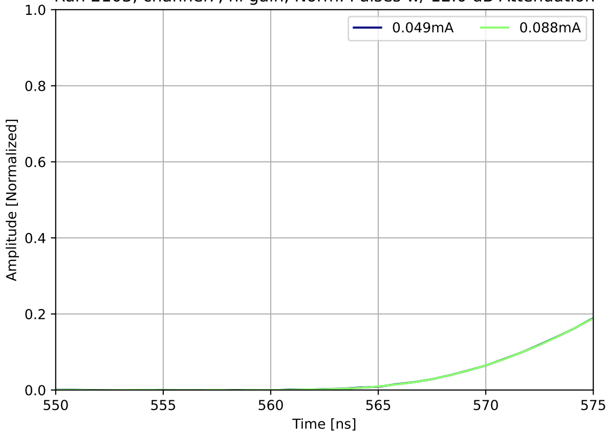
Run 2103, channel7, hi gain, Norm. Pulses w/ 12.0 dB Attenuation
