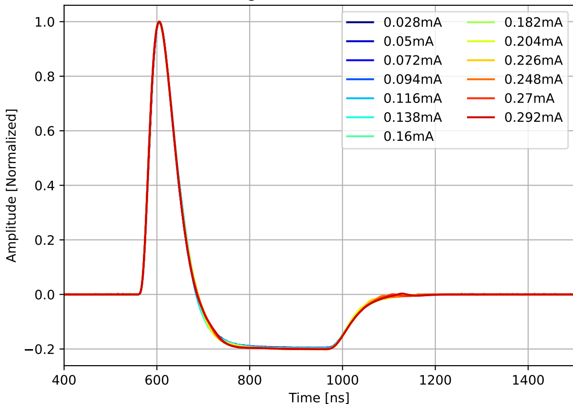
Run 2104, channel8, lo gain, Norm. Pulses w/ 17.0 dB Attenuation
