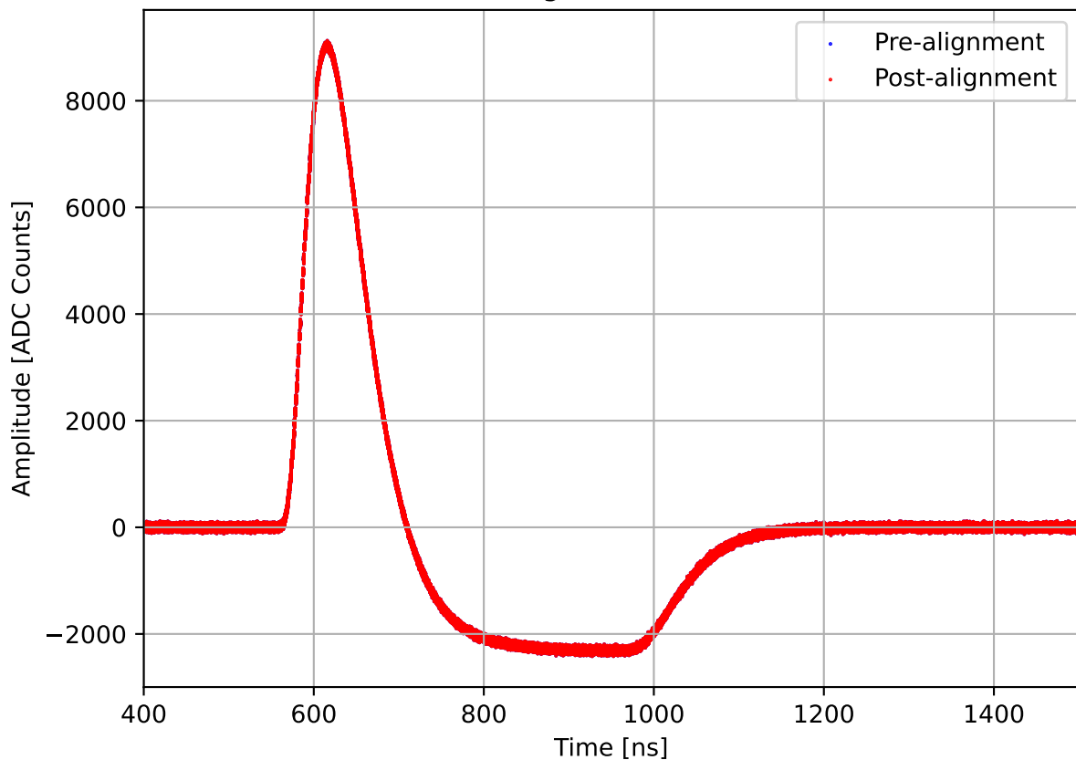
Run 2135, channel7, hi gain, Pulse w/ 7.0 dB Attenuation
