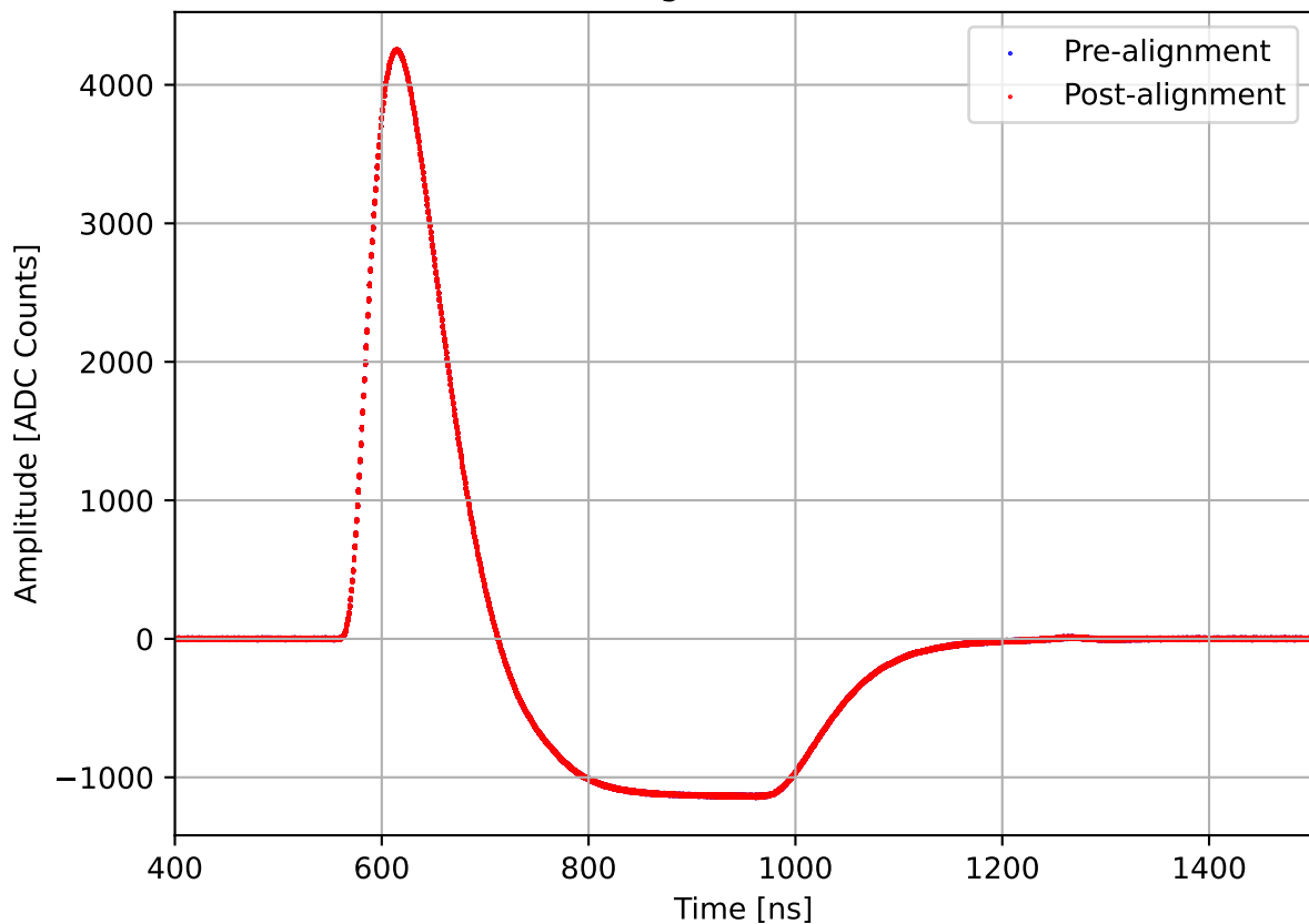
Run 2135, channel8, lo gain, Pulse w/ 7.0 dB Attenuation
