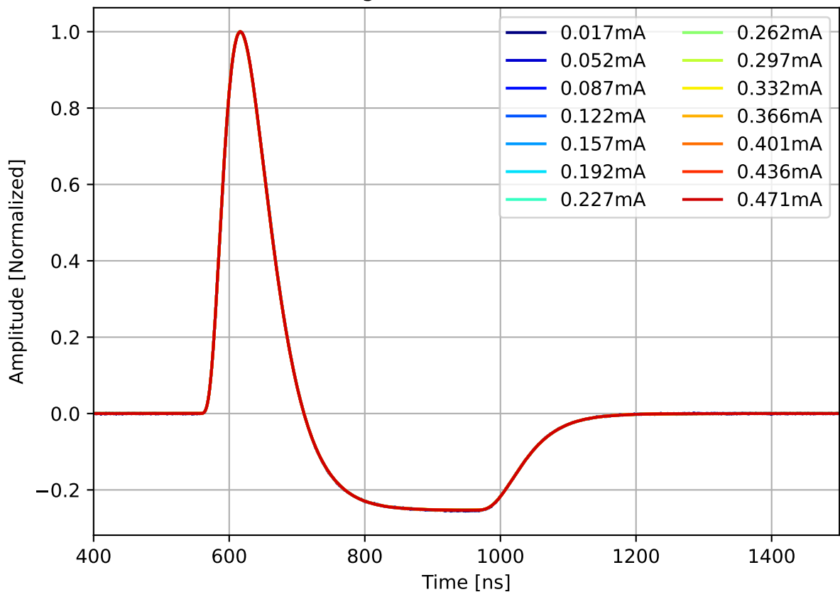
Run 2144, channel6, hi gain, Norm. Pulses w/ 27.0 dB Attenuation
