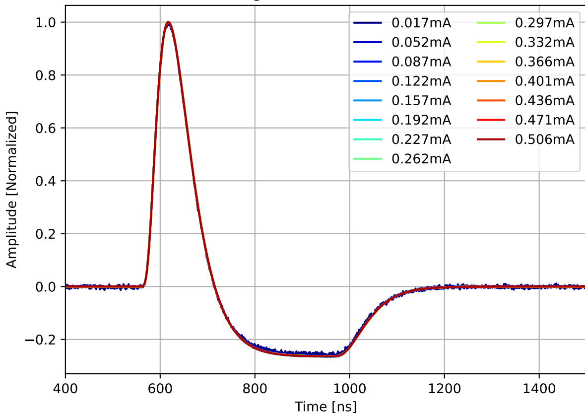
Run 2144, channel5, lo gain, Norm. Pulses w/ 27.0 dB Attenuation
