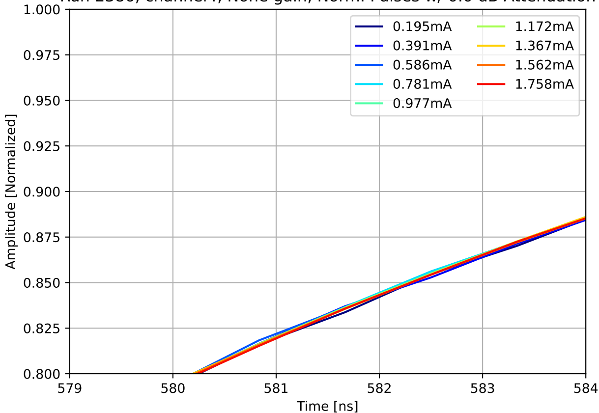
Run 2386, channel4, None gain, Norm. Pulses w/ 0.0 dB Attenuation
