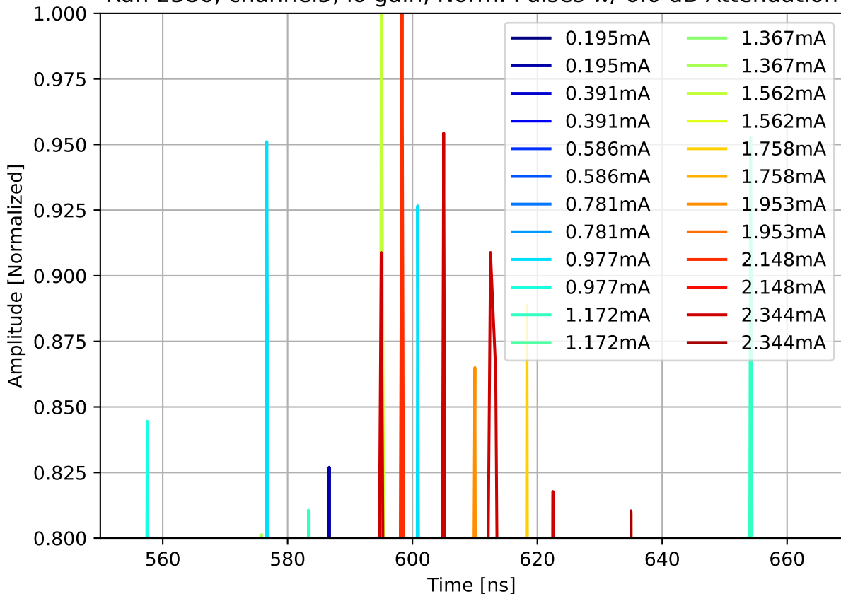
Run 2386, channel5, lo gain, Norm. Pulses w/ 0.0 dB Attenuation
