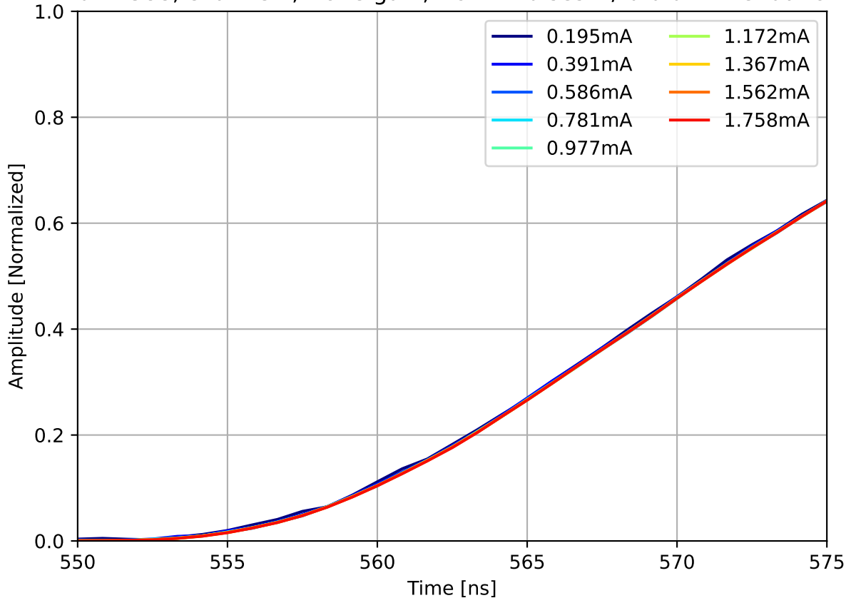
Run 2388, channel4, None gain, Norm. Pulses w/ 0.0 dB Attenuation
