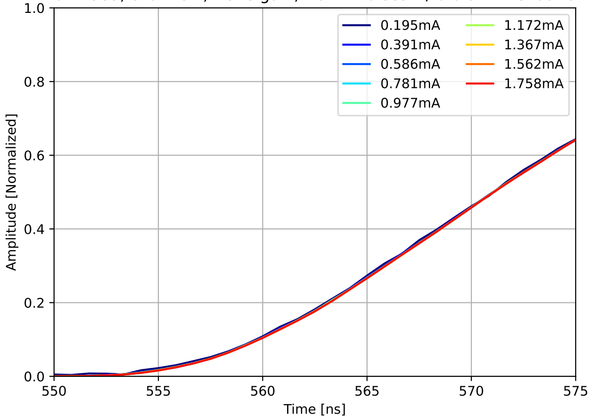
Run 2389, channel4, None gain, Norm. Pulses w/ 0.0 dB Attenuation
