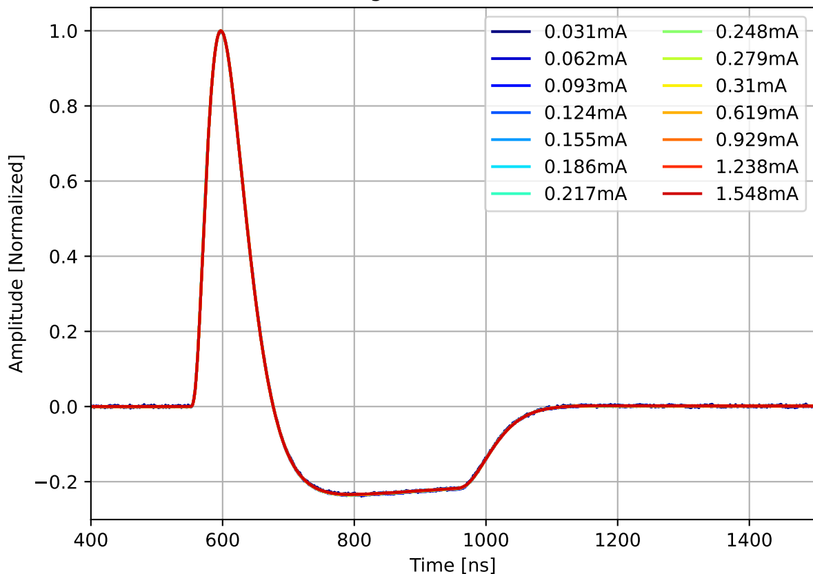
Run 2407, channel4, None gain, Norm. Pulses w/ 16.0 dB Attenuation
