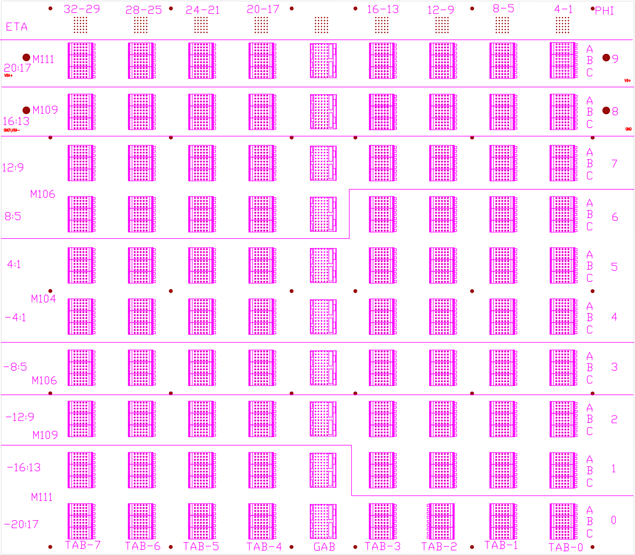
SLOT-19 SLOT-17 SLOT-15 SLOT-13 SLOT-11 SLOT-9 SLOT-7 SLOT-5 SLOT-3 THIS VIEW IS FROM THE BACK OF THE CRATE TAB-GAB BACKPLANE
