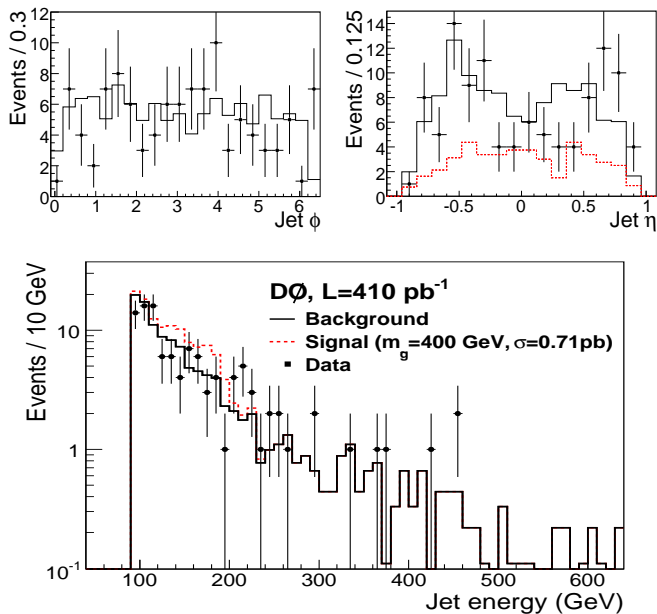
FIG. 1: A comparison of the wide-shower no-muon data (points) to the expected background from cosmic muons (solid histogram) and a simulated signal (dashed histogram).
