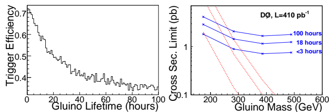
FIG. 3: Left: The trigger efficiency vs. gluino lifetime. Right: The upper limits observed on the cross section of stopped gluinos, for various assumptions of the gluino lifetime, for a \tilde{\chi}_1^0 mass of 50 GeV, along with theoretical cross sections.
