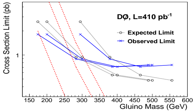
FIG. 2: The expected and observed upper limits on the cross section of stopped gluinos, assuming a 100% BR of \tilde{g} \rightarrow g\tilde{\chi}_1^0 and a small gluino lifetime ( <3 hours), for three choices of the \tilde{\chi}_1^0 mass: 50, 90 and 200 GeV, from left to right. Also shown is the theoretical cross section (dashed line), from Ref. [4], for conversion cross sections of 0.3, 3, and 30 mb (left to right).
