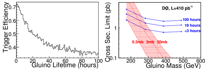
FIG. 3: Left: The trigger efficiency vs. gluino lifetime. Right: The upper limits observed on the cross section of stopped gluinos, for various assumptions of the gluino lifetime, for a \tilde{\chi}_1^0 mass of 50 GeV. Also shown are the theoretical stopped gluino cross sections (dashed lines, shaded area), from Ref. [4], for the range of assumed conversion cross sections.
