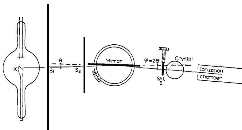
Fig. 1. Apparatus for studying the total reflection of X-rays.
