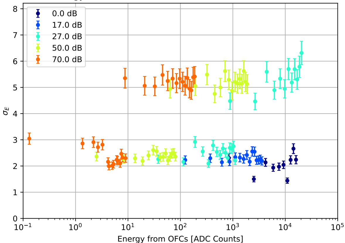
Energy Resolution, AWG Noise Subtracted (80% of DR)
