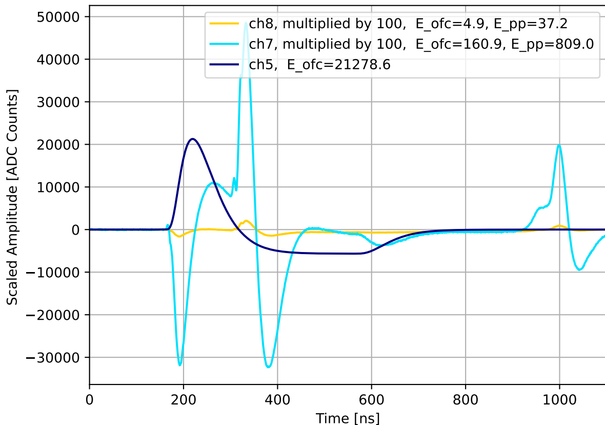
Run 2139, channel5, Crosstalk Pulses w/ 0.0 dB Attenuation
