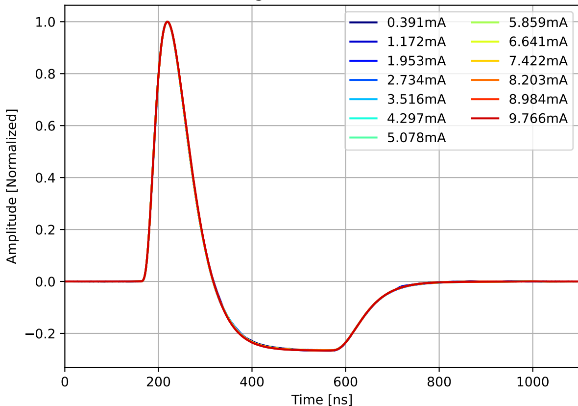
Run 2139, channel5, lo gain, Norm. Pulses w/ 0.0 dB Attenuation
