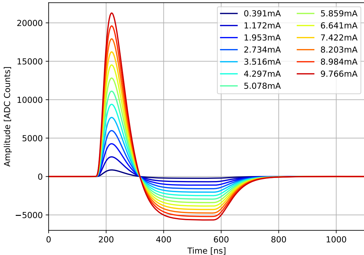
Run 2139, channel5, lo gain, Pulses w/ 0.0 dB Attenuation
