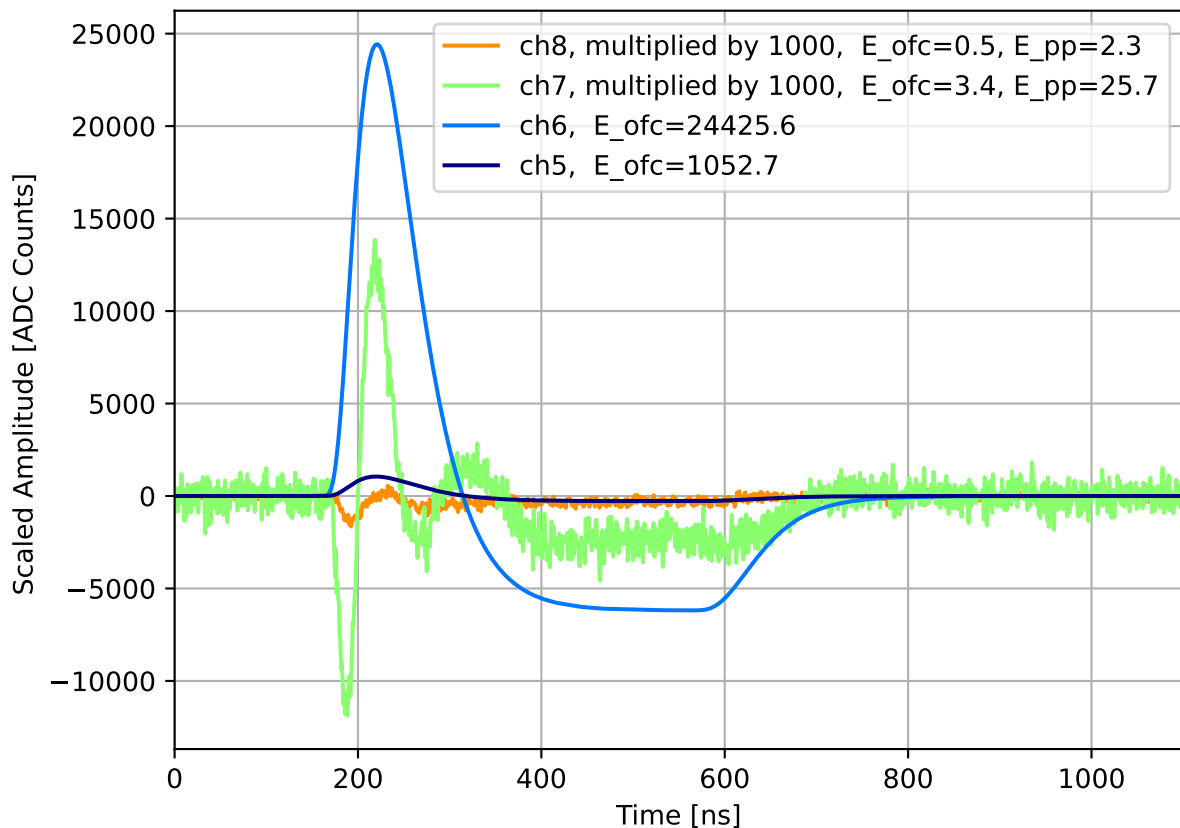
Run 2144, channel6, Crosstalk Pulses w/ 27.0 dB Attenuation
