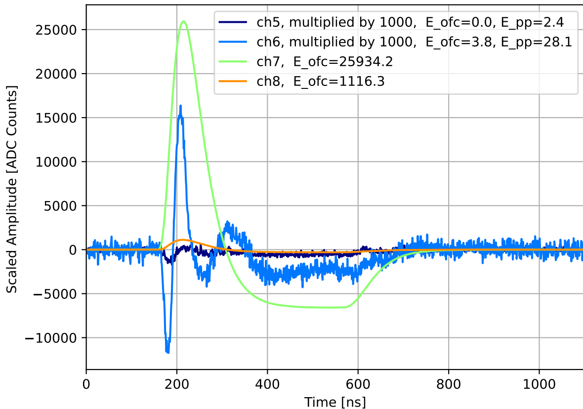
Run 1981, channel7, Crosstalk Pulses w/ 27.0 dB Attenuation
