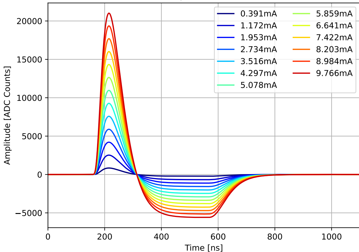
Run 1978, channel8, lo gain, Pulses w/ 0.0 dB Attenuation
