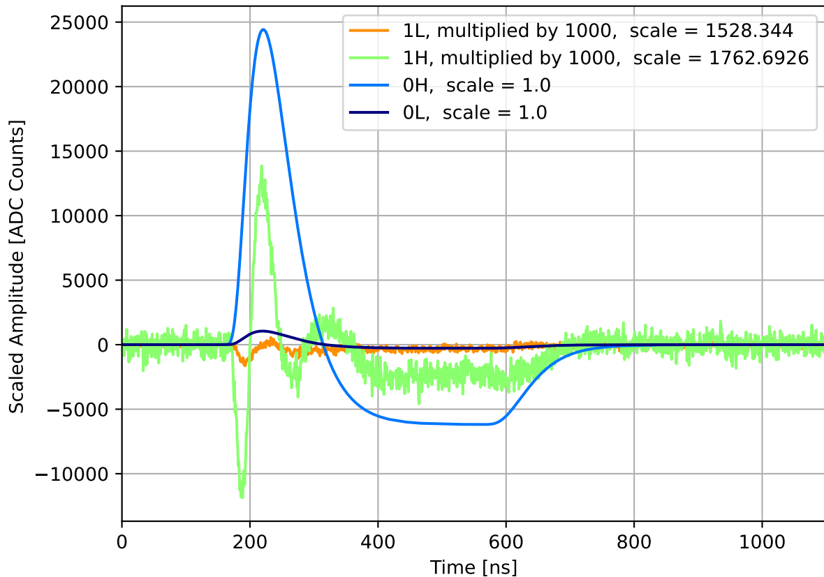
Run 2144, 0H, Crosstalk Pulses w/ 27.0 dB Attenuation
