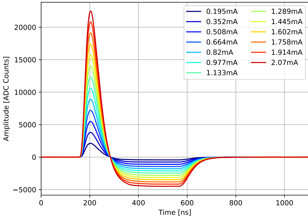
Run 2036, channel5, lo gain, Pulses w/ 0.0 dB Attenuation
